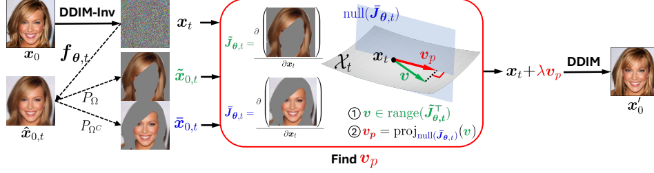
Figure 3: Illustration of the unsupervised LOCO Edit for unconditional diffusion models. Given an image \mathbf{x}_0 , we perform DDIM-Inv until time t to get \mathbf{x}_t , and estimate \hat{\mathbf{x}}_{0,t} from \mathbf{x}_t . After masking to get the region of interest (ROI) \tilde{\mathbf{x}}_{0,t} and its counterparts \bar{\mathbf{x}}_{0,t} , we find the edit direction \mathbf{v}_p via SVD and nullspace projection based on their Jacobians (Algorithm 1). By denoising \mathbf{x}_t + \lambda \mathbf{v}_p , an image \mathbf{x}'_0 with localized editing is generated. In this paper, the variables and notions related to ROI, nullspace, and final direction are respectively highlighted by green, blue, and red colors.
