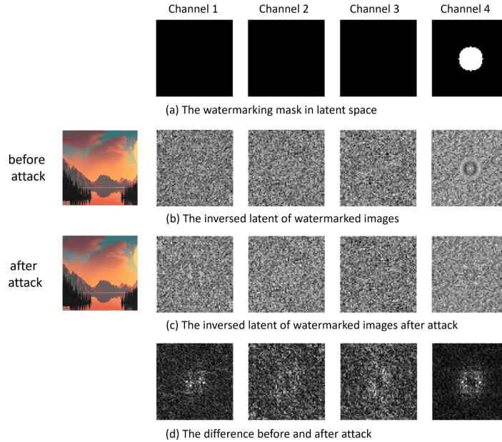
Figure 22. Visualization of AdvCls-WM1&WM2 attack. (a) and (b) are the same as that in Figure 21. (c) shows the inversed latent after the attack, where the watermark vanishes instead of changing to another watermark. (d) shows the magnitude of the element-wise difference before and after the attack. The attack not only perturbs the watermark part but also other features. The average magnitude change of the watermark-part and non-watermark-part is also around 2:1. Although the surrogate detector is trained to classify two different watermark messages. The attack based on it cannot change the watermark message from one to another but can effectively disturb the watermark.
