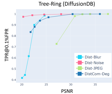
(b) Degradation distortions (PSNR ↑)
