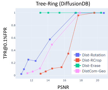
(a) Geometric distortions (PSNR ↑)
