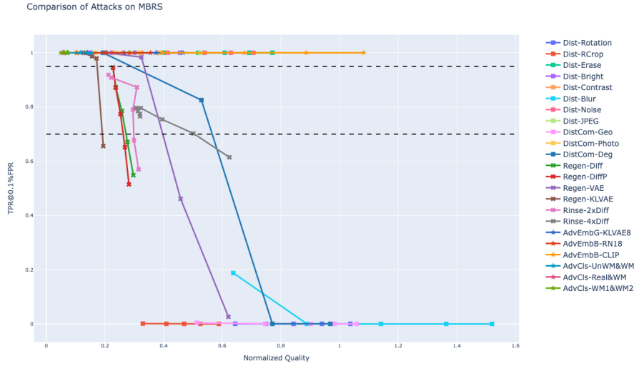
Figure 32. Stress test results for MBRS. It is vulnerable to certain distortion attacks (resized-cropping, blurring, rotation, combo distortions) and regeneration attacks, but robust against other distortions (JPEG compression, brightness/contrast, random erasing, noise) and adversarial attacks.
