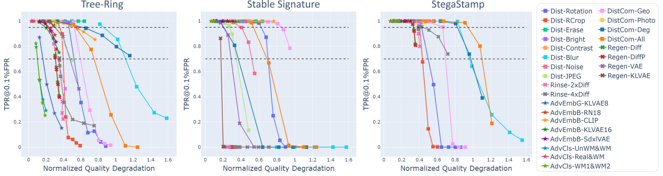
Figure 7. Unified performance vs. quality degradation 2D plots under detection setup. We evaluate each watermarking method under various attacks. Two dashed lines show the thresholds used for ranking attacks.
