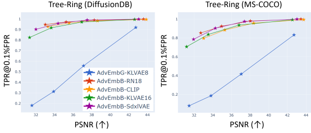
Figure 4. Adversarial embedding attacks target Tree-Ring at strengths of \{2/255, 4/255, 6/255, 8/255\} . Tree-Ring shows vulnerability to embedding attacks, especially when the adversary can access the VAE being used.
