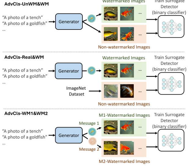
Figure 5. Three settings for training the surrogate detector. The Generator is the victim generator under attack. We externalize the watermarking process for simplicity, but it could be in-processing watermarks. After training the surrogate detectors, the adversary performs PGD attacks on them to flip the labels.
