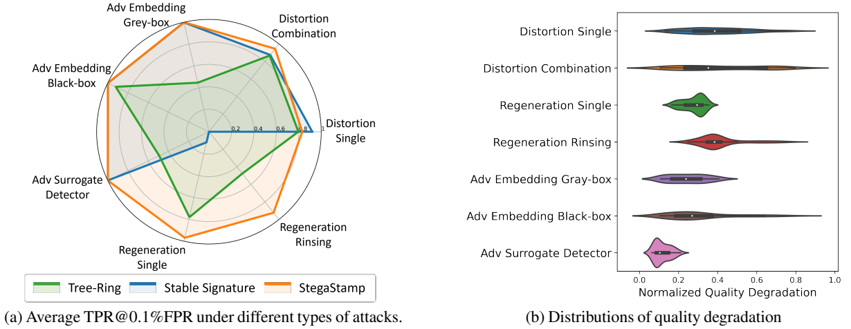
Figure 8. (a) Detection performance of three watermarks after attacks, measured by Average TPR@0.1%FPR with lower values (near center) indicating higher vulnerabilities. (b) The distribution of quality degradation. The lower, the better.
