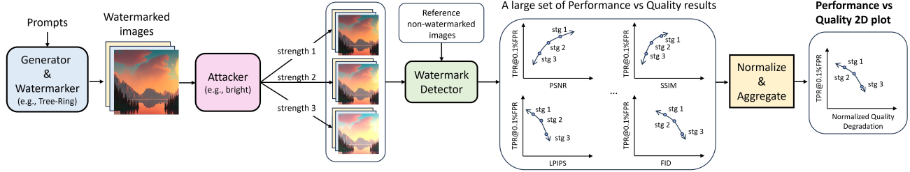
(a) Evaluation of a single attack on a watermarking method. We first attack watermarked images over a variety of strengths (also labeled 'stg'). Then, we evaluate the detection performance ( \text{TPR}@0.1\%\text{FPR} ) and a collection of image quality metrics such as PSNR and plot a set of performance vs. quality plots. By normalizing and aggregating these quality metrics, we derive a consolidated 2D plot that represents the overall performance vs. quality for the evaluation.
