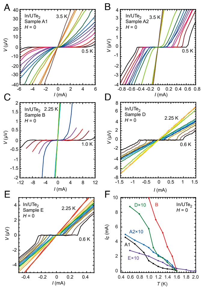
Fig. 2. Nonzero Josephson coupling in In/ UTe_2 junctions prepared on (001) and (0–11) surfaces. (A–E) Voltage ( V ) vs. current ( I ) curves for sample A1 at fixed temperatures T = 0.5, 0.7, 0.9, 1.0, 1.1, 1.2, 1.3, 1.4, 1.5, 1.6, 1.7, 2.5, 3.0 , and 3.5 K, sample A2 at T = 0.5, 0.7, 0.9, 1.0, 1.1, 1.2, 1.3, 1.4, 1.5, 1.6, 2.5, 3.0 , and 3.5 K, sample B at T = 0.6, 0.7, 0.8, 0.9, 1.0, 1.1, 1.2, 1.3, 1.4, 1.5, 1.6, 1.7 , and 2.25 K, sample D at T = 0.6, 0.8, 1.0, 1.1, 1.2, 1.3, 1.4, 1.5, 1.55, 1.6, 1.8, 1.9, 2.0 , and 2.25 K, Sample E at T = 0.6, 0.8, 1.0, 1.1, 1.2, 1.3, 1.4, 1.5, 1.6, 1.8, 1.9, 2.0 , and 2.25 K, respectively, showing the presence of finite Josephson coupling. Samples A1 and A2 were prepared on the same crystal surface while sample B was prepared on a different crystal surface, with the same (001) orientation. Samples D and E were prepared on cleaved crystal surfaces of different crystals with (0–11) orientation. The Josephson coupling vanishes at T_c \approx 1.6 K for samples A1, A2, B, and D, and for sample E, 2.0 K. (F) I_c(T) for samples A1, A2, B, D, and E. The I_c for samples A2, D, and E are multiplied by 10 for clarity.
