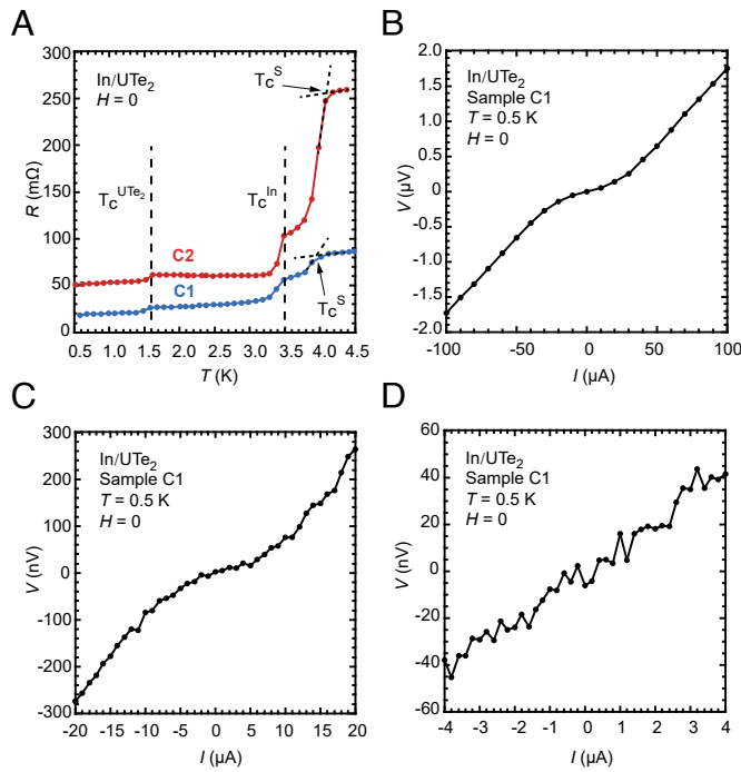
Fig. 3. Absence of Josephson coupling in In/UTe 2 junctions prepared on (1–10) surface. (A) R(T) curves measured at I = 100 \mu\text{A} in zero magnetic fields for both samples C1 and C2. Resistance drops at 1.6 and 3.4 K correspond to the T_c 's for UTe 2 and In, respectively. The feature seen near 4 K is discussed in the main text. (B–D) V - I curves for sample C1 at T = 0.5 \text{ K} measured in decreasing ranges of current. No zero-voltage currents were seen down to the smallest measurement currents.
