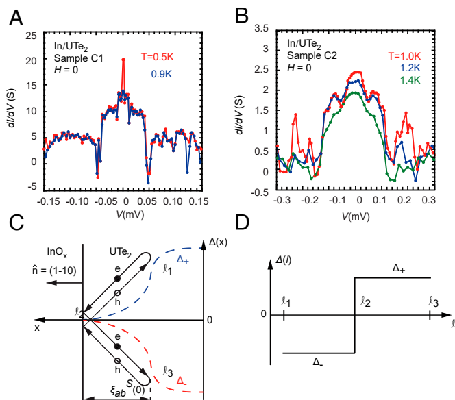
Fig. 4. Quasiparticle tunneling spectra. (A) dI/dV vs. V for sample C1 at T = 0.5 and 0.9 K with the normal-state contribution subtracted (the spectrum obtained at 2.0 K is treated as the normal-state contribution). (B) dI/dV vs. V for sample C2 at T = 1.0, 1.2, 1.4 K with normal-state contribution obtained at 1.6 K subtracted. (C) Schematic illustrating the formation of Andreev surface bound states (ASBSs) in which an electron is Andreev reflected as a hole and reflected off the surface of the crystal (remaining as a hole) before being Andreev reflected again to emerge as an electron. Here, \Delta_+(x) and \Delta_-(x) are OPs for electrons and holes traveling in opposite directions and \Delta_+ = \Delta_- = 0 at l_2 . The superconducting coherence length \xi_{ab}^S(0) is indicated. (D) Schematic illustrating the sign change of the OP along the semiclassical trajectory. The superconducting energy gap vanishes at the surface where the OP changes sign.
