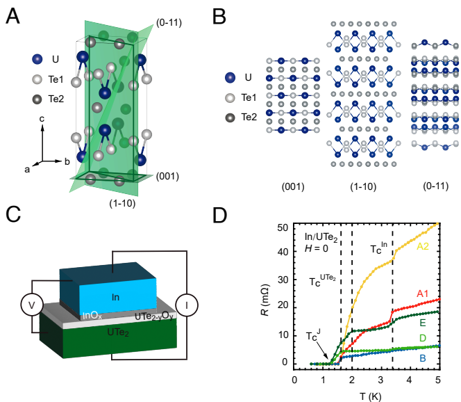
Fig. 1. Crystal structure and tunneling junction preparation. (A) Crystal structure of UTe_2 featuring the space group Immm (#71) with orthorhombic point group of D_{2h} . (B) Schematics of crystalline surfaces of (001), (1–10), and (0–11) showing very different atomic arrangements. (C) Schematic for an In/UTe_2 Josephson junction prepared on a flat surface of UTe_2 . (D) Curves of sample resistance ( R ) vs. temperature ( T ) in zero magnetic field measured at I_m = 200, 100, 500, 100, and 100 \mu A for Samples A1, A2, B, D, and E, respectively. Drops seen at 1.6 K (2.0 K) and 3.4 K correspond to the T_c 's for UTe_2 and In , respectively (see SI Appendix, Fig. S2D for the small drops at 3.4 K in Samples B and D).
