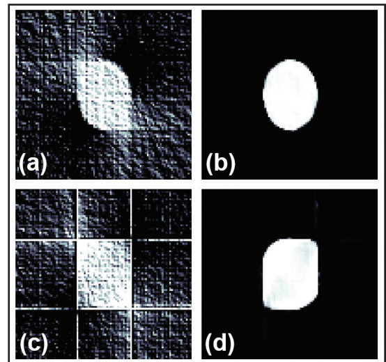
Figure 1. Direct reconstruction and network output for ellipse data (which is in the training distribution) and rectangle data (which is not). 1a. Direct reconstruction of an ellipse. 1b. Network output from the data in 1a. 1c. Direct reconstruction of a rectangle. 1d. Network output from the data in 1c. Figure courtesy of Tim Roith.
