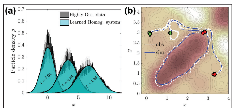
Figure 3. Coarse graining in action. 3a. Homogenization of a highly oscillatory Fokker-Planck equation from particle data. 3b. Reduction of noisy, coupled, charged particle motion (in white) to coarse-grained Hamiltonian dynamics (in blue), including inference of background electric potential \hat{V}_E (contours). Particles begin at the green markers and end at the red markers. Note the proximity of the full dynamics (circles) to the coarse-grained model (diamonds). Figure courtesy of Daniel Messenger and inspired by [4, 6].
