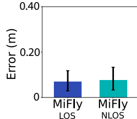
Fig. 8: Impact of Non-Line-of-Sight on Accuracy The 10 th , 50 th , and 90 th pctl of the 3D errors of MiFly in LOS&NLOS.
