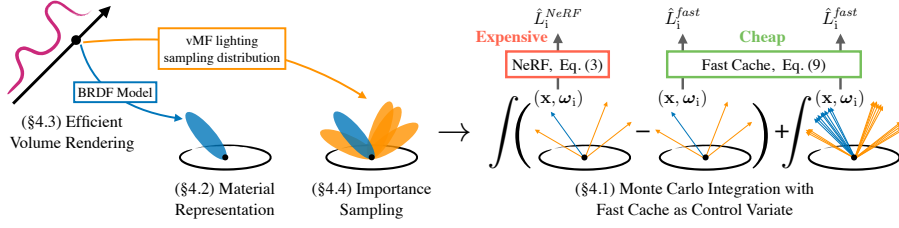
Fig. 2: Our pipeline for physically-based inverse rendering combines volume rendering with physically-based Monte Carlo rendering to recover geometry, materials, and lighting. We first use an estimator (Equation 11) to approximate the volume rendering integral (Equation 2) with only a single sample point per ray. Given this sample point, we use a spatially-varying mixture-of-vMFs (Section 4.4) to importance-sample directions based on the distribution of incoming radiance. We then produce a low-variance estimate of the rendering equation (Equation 4) using a NeRF as a radiance cache, and a fast cache approximation of the NeRF (Equation 9) that is far less expensive to evaluate.
