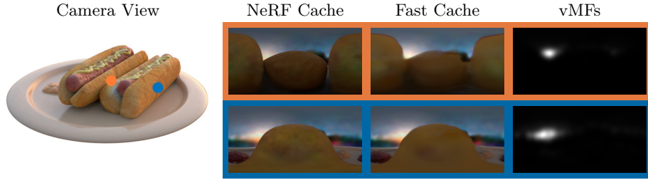
Fig. 5: ( left ) We choose two points on the hotdog for which to visualize distributions of incoming radiance. ( right ) We show (a) incoming radiance from the NeRF cache, which is high quality but slow to evaluate, (b) incoming radiance from the fast cache, which is slightly lower quality but fast to evaluate, and (c) the probability density of the spatially-varying mixture of vMFs, which is able to capture occlusions in the incoming radiance distribution.
