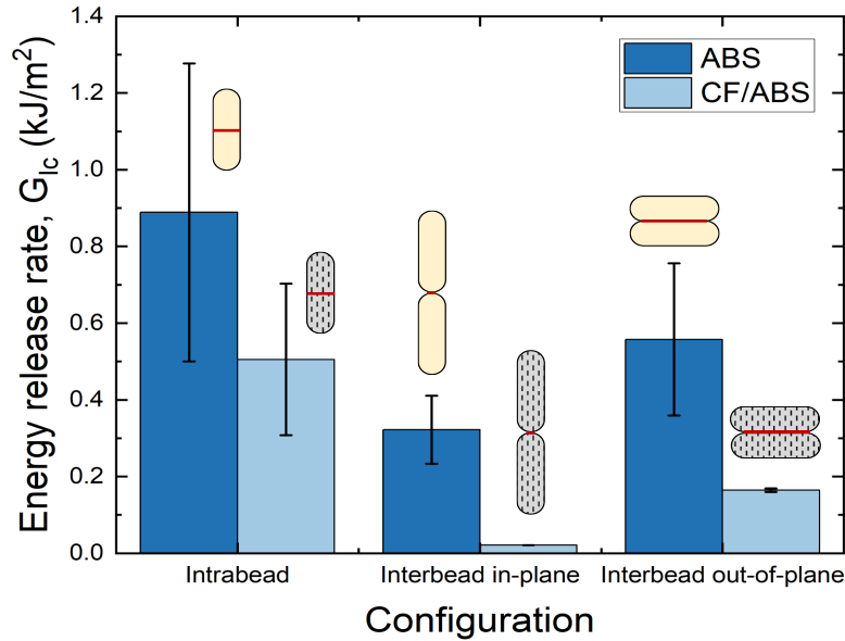
Figure 6: Comparison of ‘pure’ strain energy release rate between ABS and CF/ABS obtained from three single-bead test configurations.
