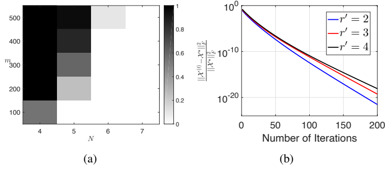
Figure 6: Performance comparison of RGD for TT format tensor completion, (a) for different N and m with d = 4 , r = 2 , and \gamma^2 = 0 , (note that for N = 4 in (a), m = 256 has been chosen when m \geq 300 ), (b) for overparameterized tensor completion where N = 3 , d = 30 , r = 2 , and m = 20000 .
