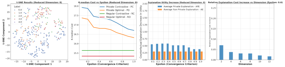
Figure 1: A visualization of our dataset (Heart Disease dataset from the UCI ML Repository), projected into an 8-dimensional space. (a) t-SNE of our data. (b) Comparison of k-medial clustering with fixed and non-fixed centroids, both private and non-private. (c) Bar graph showing contrastive explanation differences for differential private and non-private k-medial with a fixed centroid. (d) We fix the privacy budget of 0.6 while demonstrating the contrastive explanation across various dimensions.
