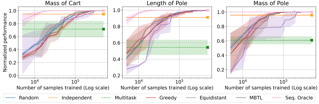
Figure 26: Comparison of normalized generalized performance of all target tasks: Cartpole.
