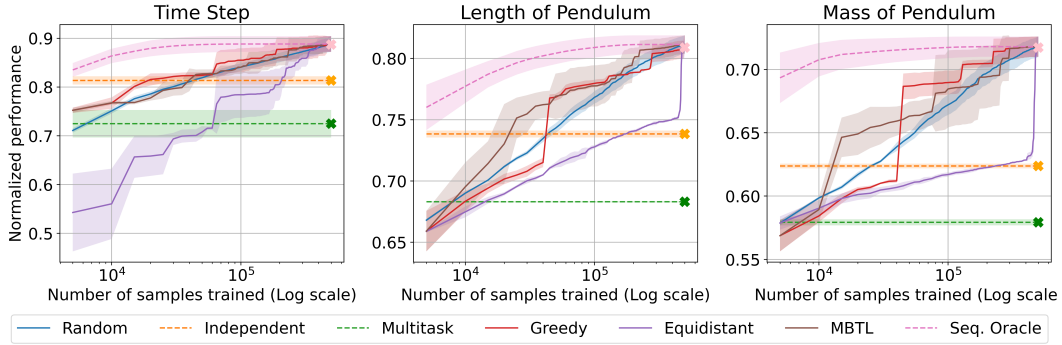
Figure 30: Comparison of normalized generalized performance of all target tasks: Pendulum.
