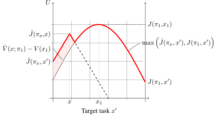
Figure 11: Step for choosing x_2 that maximizes the estimated marginal improvement ( \hat{V}(x; \pi_1) - V(x_1) ). \hat{V}(x; \pi_1) corresponds to the red area under the red line and V(x_1) as the area under J(\pi_1, x') .
