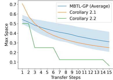
Figure 4: Empirical results of the restriction of search space by MBTL compared to two examples from Corollaries 2.1 and 2.2.
