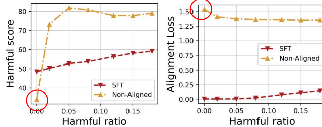
Figure 5: The circled data point shows that the non-aligned model finetuned on a clean dataset have a relatively lower harmful score and a higher alignment loss. The used fine-tuning dataset is a SST2, a sentiment classification dataset.
