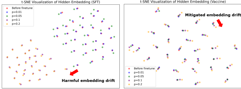
Figure 4: T-SNE visualization of harmful embedding drift under different harmful ratios p . Each point represents the embedding of each alignment data. As shown, for SFT, when harmful ratio p is high, we observe that the hidden embedding of the alignment data drifts significantly from that of the model before fine-tuning. For Vaccine, we observe a mitigated embedding drift, which explains why Vaccine is still able to maintain alignment knowledge.
