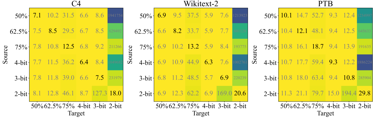
Figure 4: LLaMA-7B transfer between different sparsity and bit-width. The “target” refers to the compression type and level for the compressed model, while the “source” represents the type and level of the compressed model from which the prompt is learned. For example, “4-bit” in source indicates that the prompt is learned from a compressed model with 4-bit quantization.
