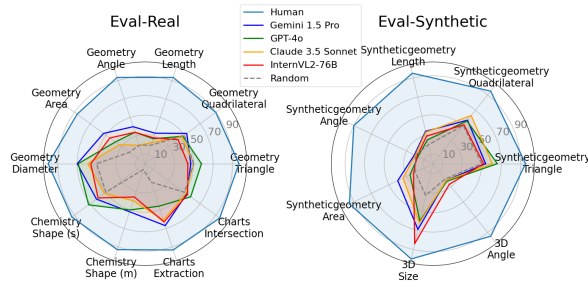
Figure 2: LVLMs perform poorly on VisOnlyQA, while human performance is nearly perfect. Table 4 provides detailed results.
