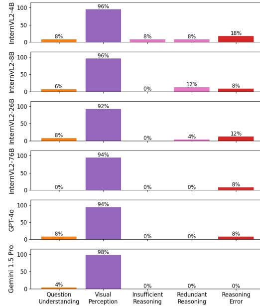
Figure 4: Error categories in chain-of-thought reasoning by LVLMS on VisOnlyQA-Eval-Real. Almost all errors are visual perception errors, verifying that our dataset evaluates the geometric perception of LVLMS independent of other capabilities. Each response can include multiple categories of errors.
