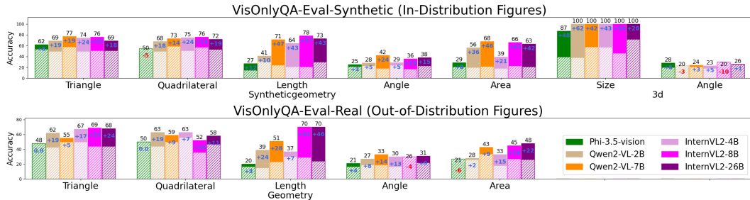
Figure 5: Accuracy after fine-tuning on VisOnlyQA-Train. We evaluate on VisOnlyQA-Eval-Synthetic, which is generated from the same distribution as the training data, and VisOnlyQA-Eval-Real, which includes images from different distributions. The numbers above the bars represent the accuracy after fine-tuning, and the ones inside the bars represent the improvements from the original models (white bars with hatches). Details are in Table 10.
