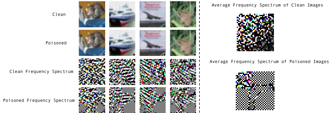
Figure 14: Visualization of the DCT of the clean images and poisoned images.
