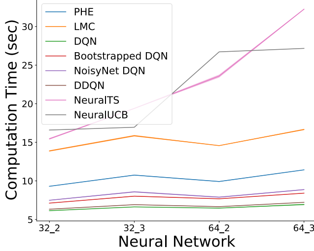
Figure 8: Computation time with different exploration strategies. Note that the x -axis indicates the neural network size, i.e., 32_2 implies two layers with 32 neurons in each layer.
