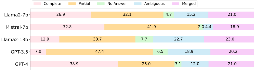
Figure 4: Distribution of answer categories (%) under Gold Only setting. Different LMs show different failure modes.
