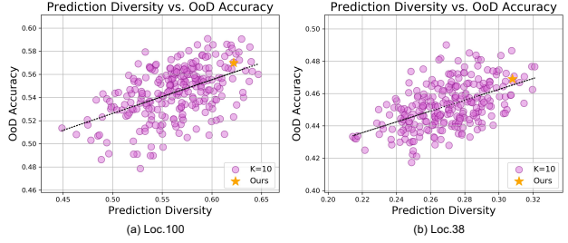
Figure 4. Visualization of prediction diversity vs. out-of-distribution accuracy on Terra Incognita . Each circle denotes a sub-ensemble with a size of 10 (half the size of the ensemble pool). The sub-ensemble selected by our method surpassed most of the selection combinations in terms of both prediction diversity and OoD accuracy.
