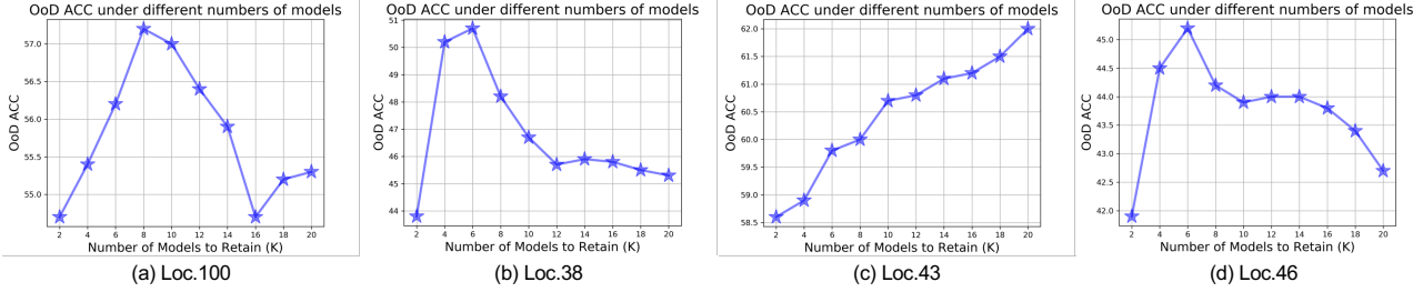
Figure 5. Ablation Study of K (Number of Models to Retain) on Terra Incognita Dataset. In locations other than “Loc.43”, the accuracy increases first and then decreases when we increase the number of models to keep ( K ). However, in “Loc.43”, the best performance is achieved at K = N = 20 . In this case, the results indicate that there is no redundancy in the ensemble pool and each model is necessary for the ensemble. Note that the accuracy on Loc.43 is the highest among all the locations. This indicates the distribution shift (between the source and target) is not as prominent as other locations. The results indicate our method yields better performance when the distribution shifts are relatively significant.
