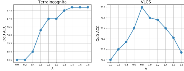
Figure 3. Ablation study on \lambda . In Terra Incognita , we found in-distribution accuracy does not contribute to the improvement. We suspect the reason is that, when distribution shift is large, the in-distribution accuracy may not be informative for OoD data. In VLCS , we found both in-distribution accuracy and OoD diversity contribute to the improvement.
