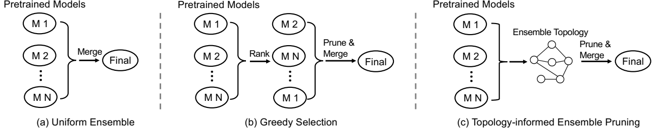
Figure 2. Overview of different strategies for ensemble pruning. Different from existing works that are tailored for in-distribution data, our proposed topology-informed ensemble pruning is capable of promoting predictive diversity and lowering generalization errors on shifted distributions with theoretical guarantees.
