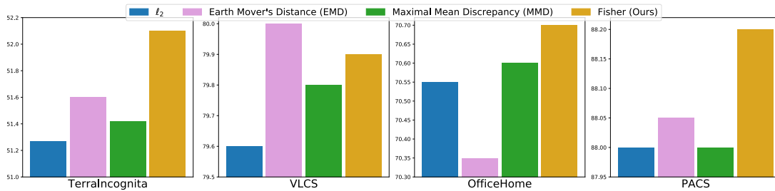
Figure 6. Accuracy (%) of alternative distance metrics for model topology construction. We compare with several common distance metrics including \ell_2 , Earth Mover’s Distance (EMD), and Maximum Mean Discrepancy (MMD). Results show Fisher is only slightly worse than EMD on VLCS and outperforms all the other metrics on other datasets. We attribute the effectiveness to Fisher’s sensitivity in capturing the parameter-output relationships (Matena & Raffel, 2022).
