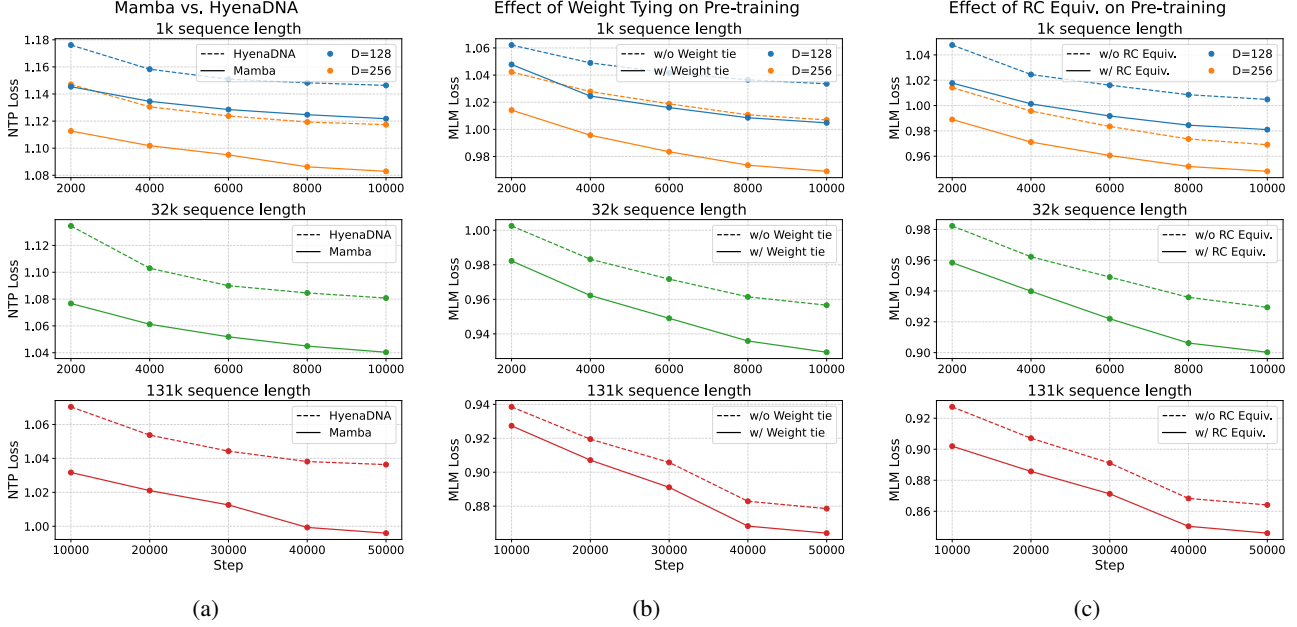
Figure 3. Pre-training test set loss. (a) For comparable model size and sequence length, Mamba attains better cross entropy loss than HyenaDNA during pre-training on the human genome. (b) Across sequence lengths, deeper models that use weight tying have better pre-training loss on the human genome. (c) Across sequence lengths, RC equivariance leads to better pre-training loss on the human genome. Note, models with a sequence length of 131k were validated less frequently to reduce overhead during pre-training. By adjusting batch size, we hold number of tokens per batch constant across varying lengths.
