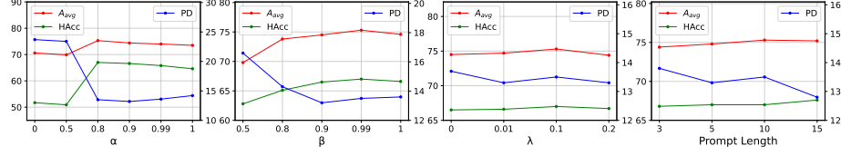
Fig. 4: Sensitive analysis of \alpha , \beta , \lambda and prompt length L_g = L_d . The average accuracy A_{avg} is reported on ImageNet-R datasets.
