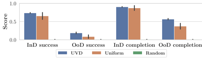
Fig. 5: Comparison with heuristic goal-labeling methods.
