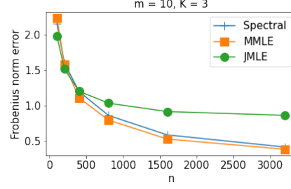
Figure 1: When the prior is correctly specified, MMLE performs as well as the spectral algorithm. JMLE is inconsistent when the number of tests is small.
