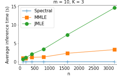
Figure 2: The spectral algorithm is much more efficient than both JMLE and MMLE.
