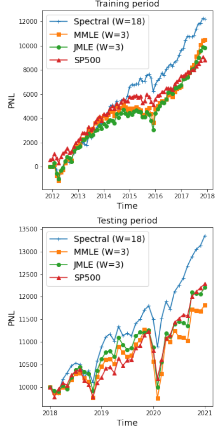
Figure 5: Cumulative PNL of trading strategies using PCM inference algorithms.
