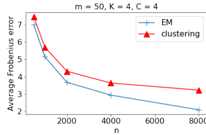
Figure 4: The Spectral-EM iterative algorithm refines the cluster-then-learn initial estimate.
