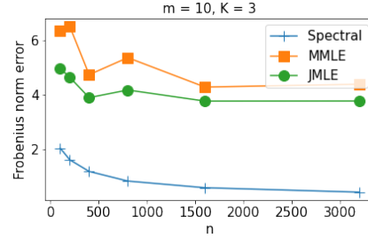
Figure 3: When the prior is mis-specified, MMLE produces inaccurate estimate.
