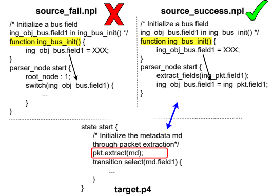
Figure 5: Different ways to initialize temporary vars.
