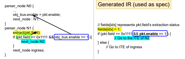
Figure 8: Predicate generation.
