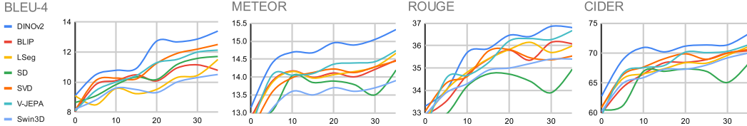
Figure 4: Evaluation curves on the ScanQA benchmark. The x -axis demonstrates models trained for different epochs. DINOv2 exhibits clearly superior performance.
