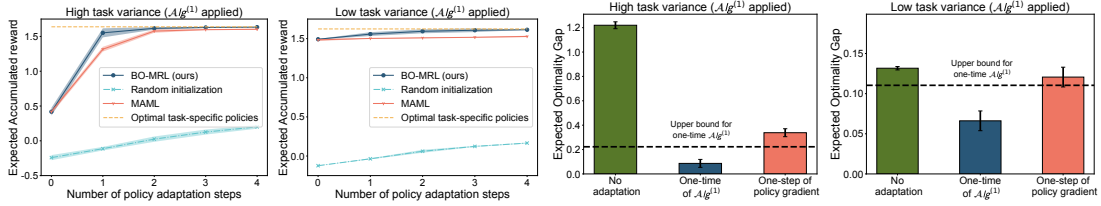
Figure 1: Results of the meta-test on Frozen Lake, where \mathcal{A}lg^{(1)} is applied. Left: Average accumulated reward across all test tasks v.s. number of policy adaptation steps; Right: Comparing the expected optimality gap by the BO-MRL and baselines with the upper bound of the accumulated reward of one-time \mathcal{A}lg^{(1)} .
