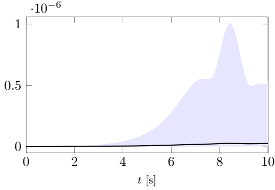
(a) Difference between prediction generated using the method in (Williams et al., 2015b) and the truncated pseudoinverse implementation of the method developed in this paper.
