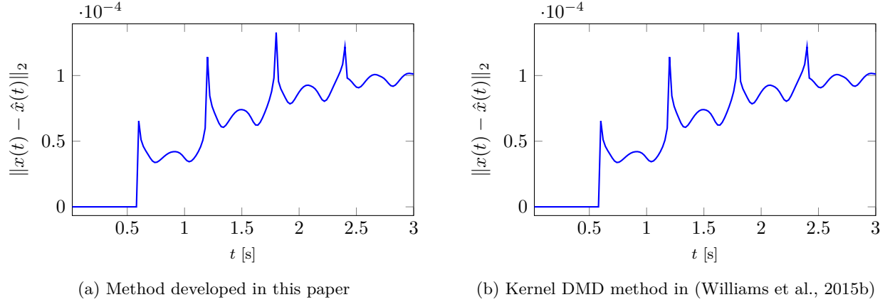
Figure 2: For the periodic flow example, this figure shows the 2-norm of the error between the true snapshots and the snapshots generated using DMD. The results for the Gaussian RBF kernel and the exponential dot product kernel are identical.
