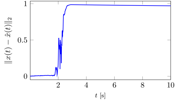
(b) Kernel DMD method in (Williams et al., 2015b)
