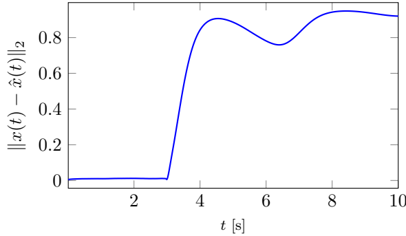
(a) Method developed in this paper
