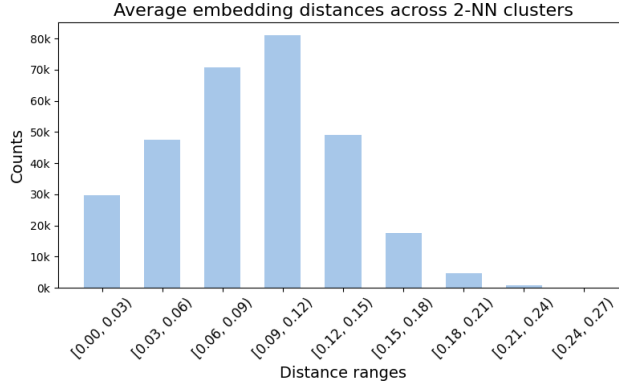
Figure 9: Average embedding distances across 2-NN clusters from our data pool. The embedding model is BAAI/bge-large-en.
