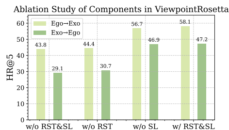
Figure 7. Ablation of components of our ViewpointRosetta.
