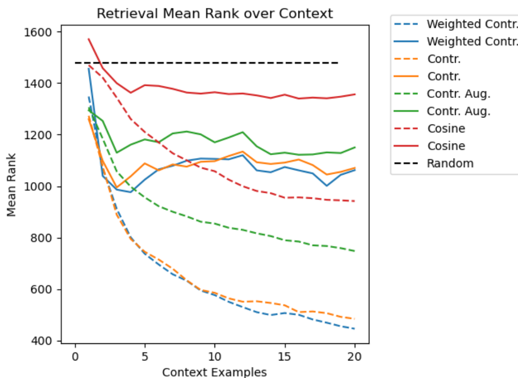
Figure 4: This figure shows the mean rank of the retrieved structure as more context synergy tuples are shown to the model. Solid lines show unknown drugs and dotted lines indicate known drugs. For visualization purposes, we use Cosine for the unknown drug and Contr. for the known drug.
