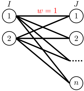
Figure 2. An example illustrating the upper bounds on Competitive Ratio (CR) for Online Capacitated Coverage Maximization (OCCM) with (\Delta, \tau) = (1, 1 - 1/e) due to Benchmark LP II.
