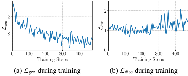
Figure 2: (On MNLI) Training the generator via \mathcal{L}_{gen} does not automatically decrease \mathcal{L}_{disc} .
