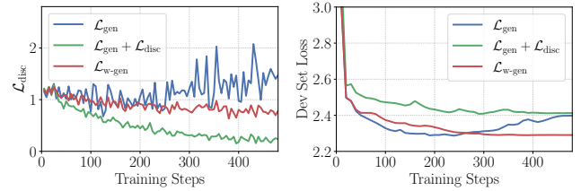
(a) \mathcal{L}_{\text{disc}} during training
