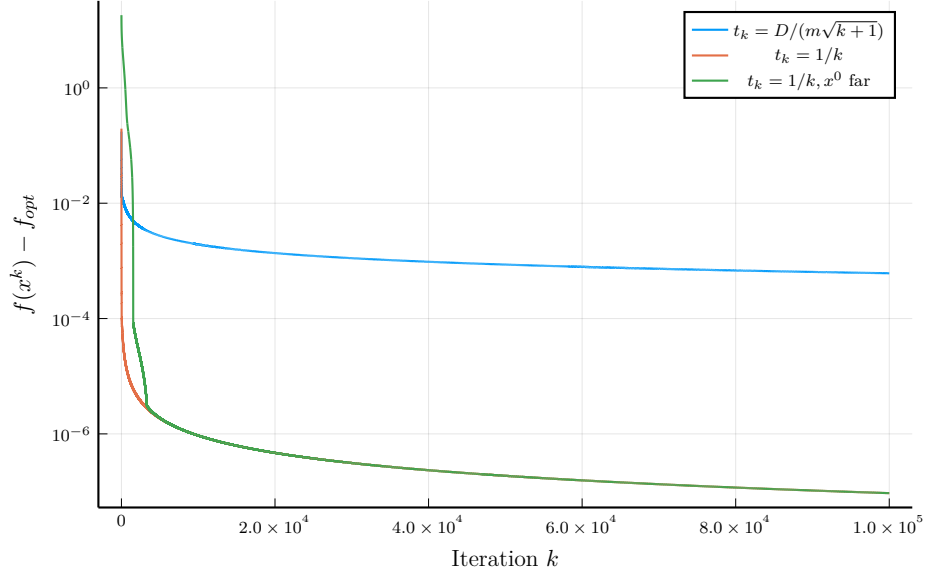
Figure 6.4: Convergence of f(x^k) to f_{\text{opt}} in Example 6.2 using two different stepsizes and choices of initial tree.
