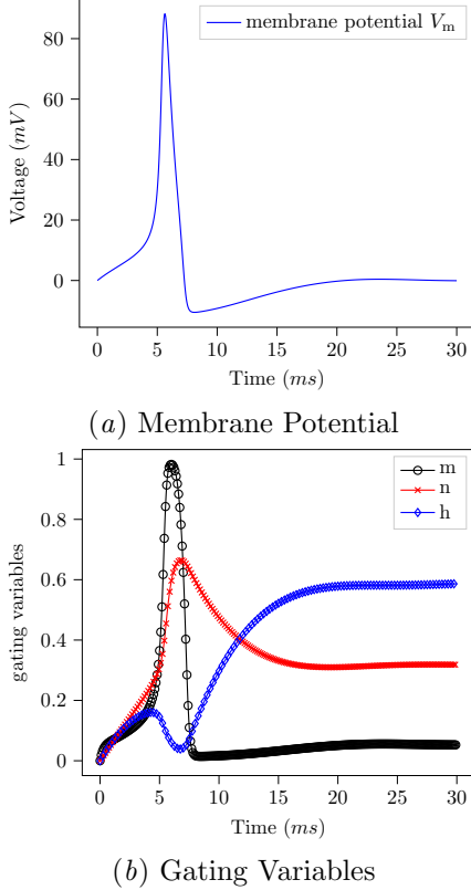
Figure 1: Evolution of the membrane potential and gating variables of normal HH equations, with no controls/stimuli, i.e., u = 0 , \forall t > 0 , and initial state \mathbf{x} = [0, 0, 0, 0]^\top .
