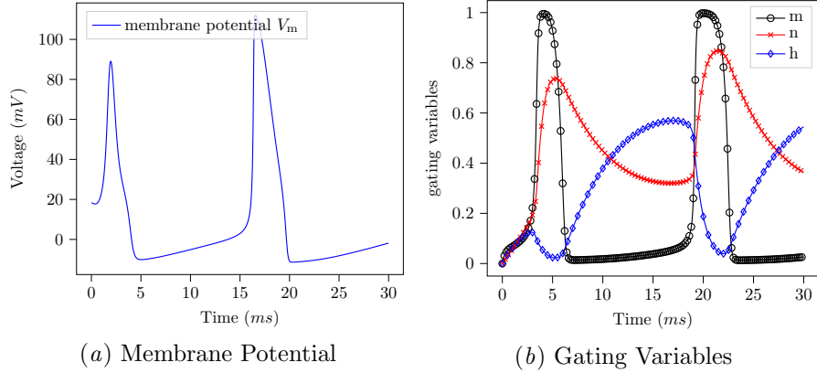
Figure 2: Evolution of the membrane potential and gating variables of pathological HH equations, with no controls/stimuli, i.e., u = 0, \forall t > 0 , and initial state \mathbf{x} = [0, 0, 0]^\top .
