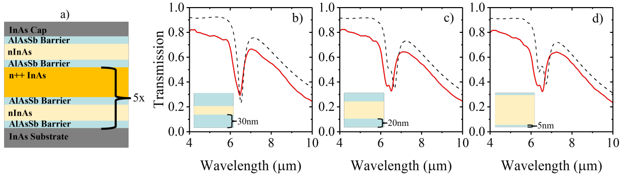
Fig. 1. (a) Dimensionless layer stack of the hyperbolic metamaterials (HMMs) studied in this work. TM-polarized transmission taken at 60^\circ plotted in red is compared to nonlocal transfer matrix calculations of primordial modes plotted in black for HMMs of varying barrier thickness with total dielectric thickness held constant [8]. Our HMM system is comprised of the periodic semiconductor material stack AlAsSb/nInAs/AlAsSb/n++InAs: (b) 30nm/20nm/30nm/80nm, (c) 20nm/40nm/20nm/80nm, and (d) 5nm/70nm/5nm/80nm.
