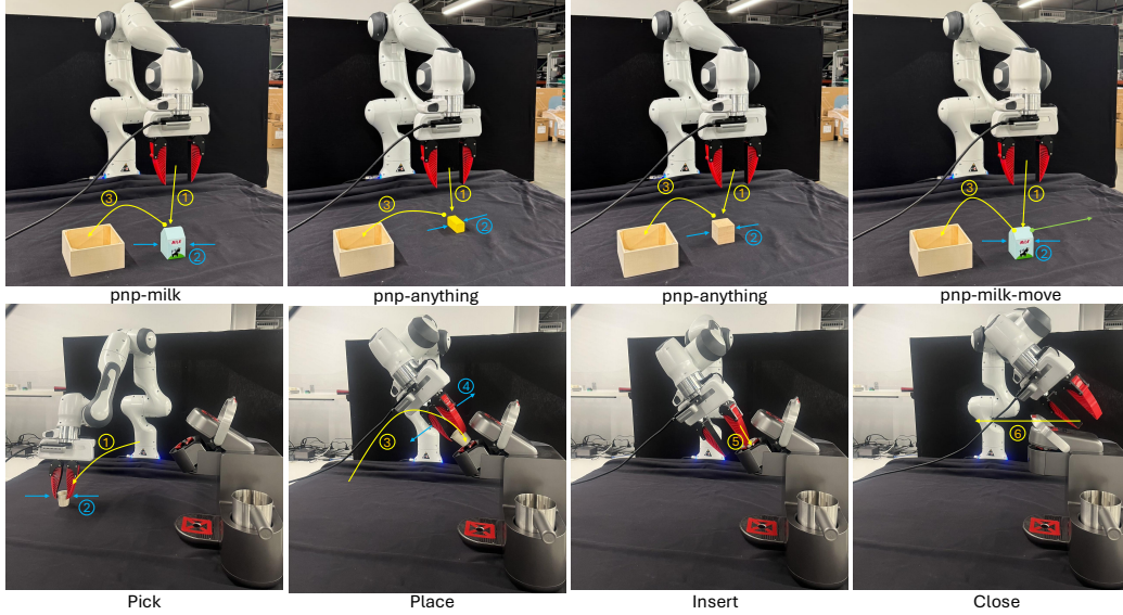
Figure 5: Real-World Experiment Illustration. In the first row, we display the setup for the pick-and-place experiments, featuring three tasks: pnp-milk , pnp-anything , and pnp-milk-move . In total, pnp-anything handles around 10 random objects as shown in Figure 8. The second row illustrates the procedure for the more challenging coffee task, where the Franka arm is tasked with locating the coffee cup, precisely positioning it in the machine’s cup holder, inserting it, and finally closing the machine’s lid.
