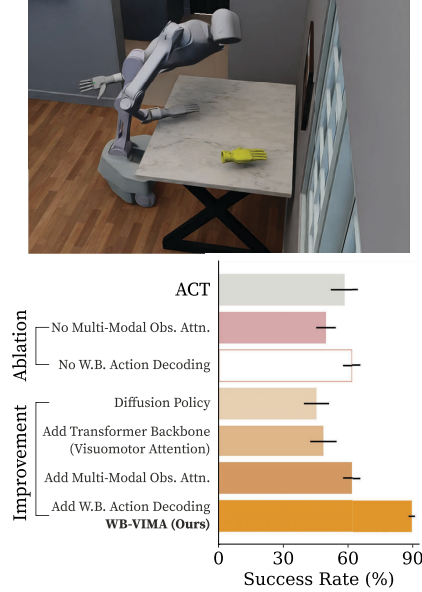
Figure 7: Simulation ablation results for “wiping table.” The robot must wipe toward the goal using whole-body motions while maintaining continuous hand contact. Results are averaged over five runs with 100 rollouts each; error bars indicate standard deviation.
