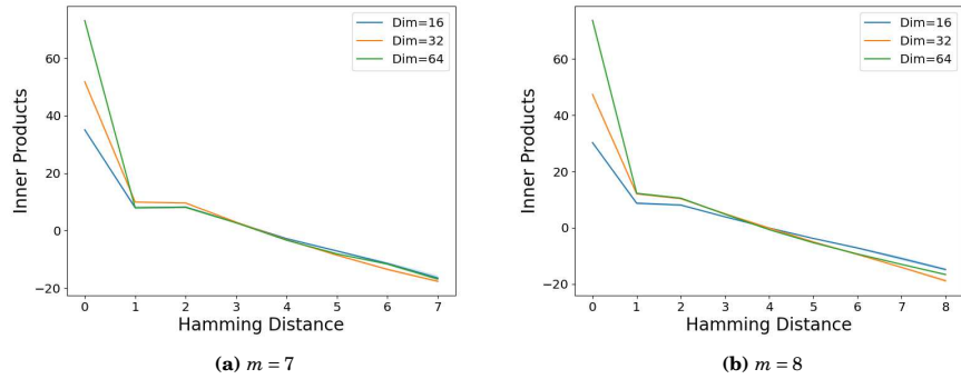
Figure C.5: The relationship between inner products of embeddings and corresponding Hamming distances of tokens can be approximated by (5.2). The graph displays the average inner product between embeddings of two tokens against the corresponding Hamming distance between these tokens. Standard errors are over 5 runs.
