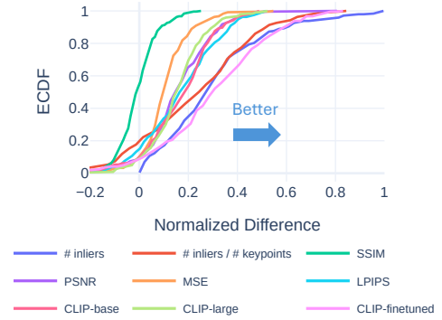
Figure 15: Discriminability of pose confidence metrics.
