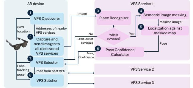
Figure 3: Localization pipeline on OpenFLAME.
