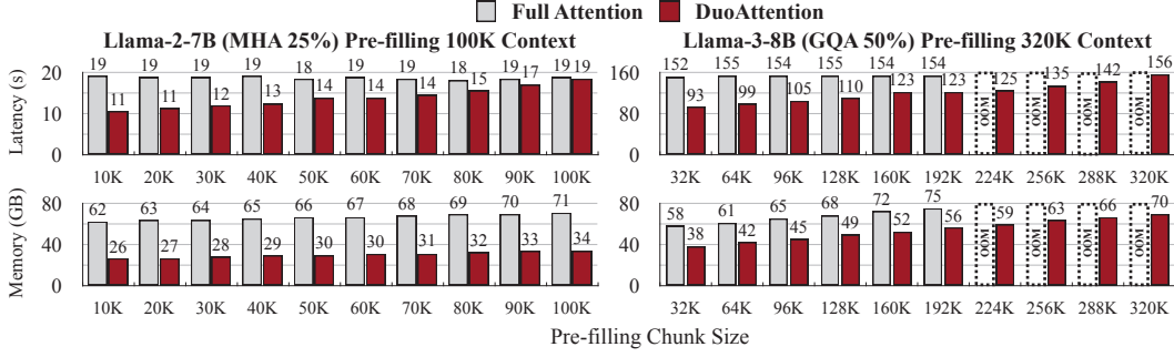
Figure 10: Pre-filling latency and memory usage of DuoAttention compared to full attention across varying pre-filling chunk sizes. DuoAttention uses a 25% retrieval head ratio for Llama-2-7B (MHA), pre-filling a context of 100K tokens, and a 50% ratio for Llama-3-8B (GQA), pre-filling a context of 320K tokens. As the pre-filling chunk size decreases, DuoAttention achieves up to 1.73\times latency reduction for MHA and 1.63\times for GQA models, with memory reductions up to 2.38\times for MHA and 1.53\times for GQA models.
