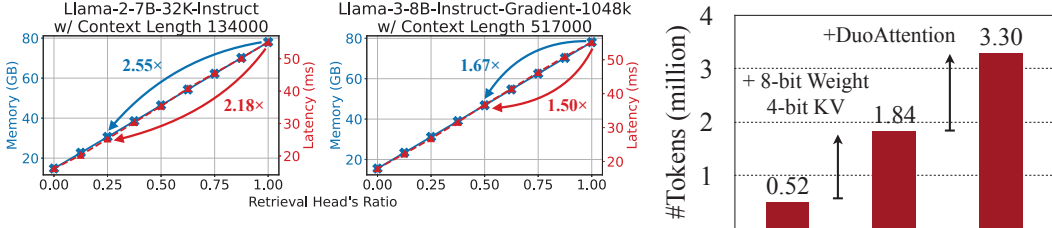
Figure 11: DuoAttention's decoding memory and latency vs. KV budget with a fixed context length. Memory and latency are reduced linearly when the ratio of retrieval heads is reduced. DuoAttention achieves up to 2.55\times memory reduction for MHA and 1.67\times for GQA models, along with up to 2.18\times latency reduction for MHA and 1.50\times for GQA models.
