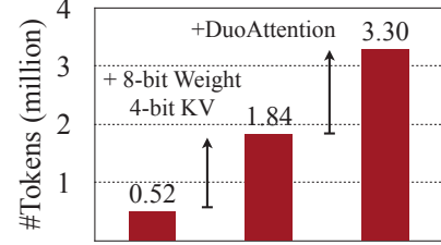
Figure 12: Combined with 8-bit weight and 4-bit KV cache quantization, DuoAttention can accommodate 3.30 million tokens on a single A100-80G GPU for the Llama-3-8B model.
