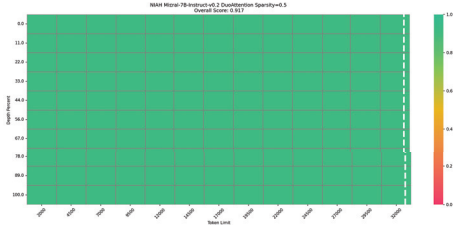
Figure 15: NIAH result on the Mistral-7B-Instruct-v0.2 model.
