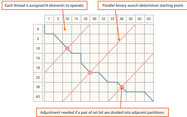
Figure 3: Performing bitwise operations between two compressed chunks on GPU. First, the chunks are divided to smaller partitions that contains an equal number of N elements, then each GPU thread can process such a partition individually.
