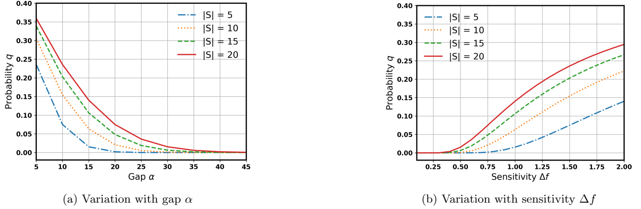
Figure 8: Variation of probability q as a function of gap \alpha_{P',P^*} in (a) and sensitivity \Delta f in (b) for different values of |S_{P',P^*}| . We set (\varepsilon, \delta) = (1, 0.01) . Additionally, for (a), we fix \Delta f = 1 and for (b), we fix \alpha_{P',P^*} = 15 .
