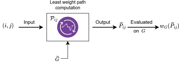
Figure 2: Evaluation Framework: Given node pair (i, j) and privatized graph \tilde{G} , a user computes the shortest path on the set \mathcal{P}_{ij} . Computation returns \tilde{P}_{ij} as the perceived shortest path, but the user decision is evaluated on original graph G incurring a cost of w_G(\tilde{P}_{ij}) and realizing bias B_{ij} = w_G(\tilde{P}_{ij}) - w_G(P_{ij}^*) .
