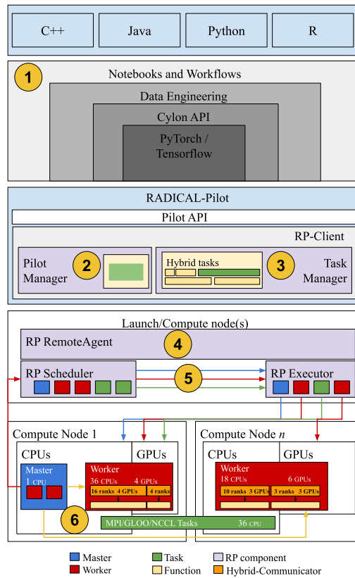
Fig. 1. Deep RC design incorporating Radical-Cylon [21] Architecture with GLOO and NCCL as communication framework. A modular design with dependent components. Segregated independent module with top-down flow from cross-platform to hardware resources. Application pipeline is incorporated with Cylon APIs and PyTorch and TensorFlow with proposed Deep RC Bridge in Fig.-2
