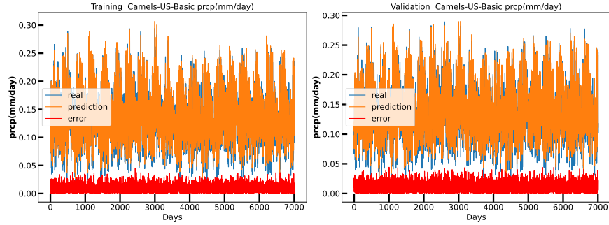
Fig. 5. Training(left) and Prediction(right) accuracy of Precipitation with Camels-US datasets [2] in LSTM Hydrology model.
