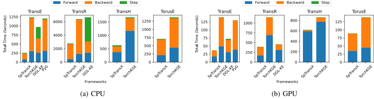
Figure 8. Breakdown of total training time for CPU and GPU on average of 7 datasets
