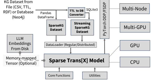
Figure 4. SparseTransX Framework
