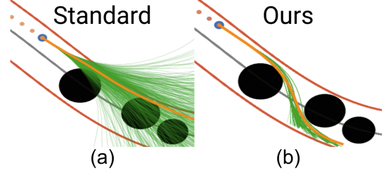
Fig. 1: Standard sampling vs. Resampling-Based Rollout (RBR) . In this AutoRally example, the blue dot samples future trajectories and computes an optimal control that avoids the black obstacles. RBR rewires all sampled trajectories to be safe, resulting in a more accurate sampling distribution. In contrast, the standard approach samples from a Gaussian distribution and wastes computation on unsafe trajectories.
