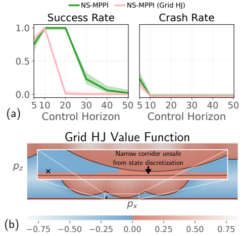
Fig. 12: Value functions from grid-based solvers suffer in multi-fidelity problems. (a) Using a value function from a grid-based HJ reachability solver results in much lower success rates at longer control horizons compared to the learned DPNCBF. (b) Due to state discretization, the narrow corridor is marked unsafe, causing the drone to be overly conservative and not cross the corridor to remain safe.
