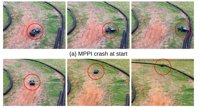
Fig. 15: Adversarial cost. With a cost function that rewards crashes, both MPPI and S-MPPI crash. Only NS-MPPI completes 10 laps collision-free.
