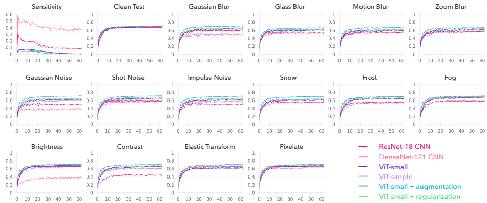
Figure 17: Comparison of the sensitivity, test accuracy on CIFAR-10 and test accuracies on various corruptions from the CIFAR-10-C dataset (see Section 7 for details) of two CNNs and two ViTs trained on the CIFAR-10 dataset, as a function of the training epochs. We also compare with ViT-small trained with data augmentation/regularization, which encourage low sensitivity (see Section 7 for discussion).
