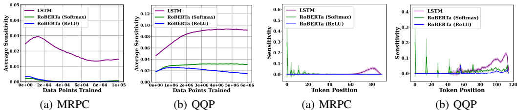
Figure 5: Sensitivity over Datapoints Trained. On both datasets, the Transformer-based model RoBERTa displays much lower sensitivity compared to LSTMs during the entire training process. RoBERTa with ReLU activation has lower sensitivity compared to its Softmax counterpart at later stages of training.
