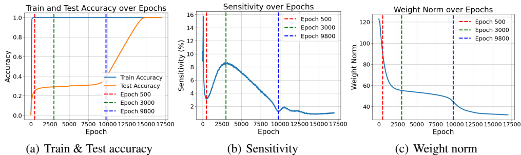
Figure 8: Sensitivity measures progress on modular addition task a + b \bmod 113 and indicates different stages of grokking.
