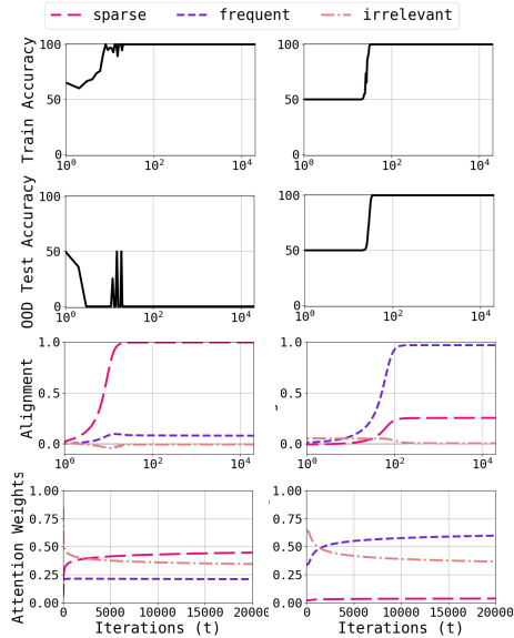
Figure 3: Train and test dynamics for a single-layer self-attention model (Eq. (3)) using the synthetic data visualized in Fig. 2; see Section 4.1 for details. Left column: the predictor that uses sparse tokens has lower sensitivity (Ex. 1 in Figure 2), Right column: the predictor that uses frequent tokens has lower sensitivity (Ex. 2 in Figure 2); see Appendix A.1 for more examples.
