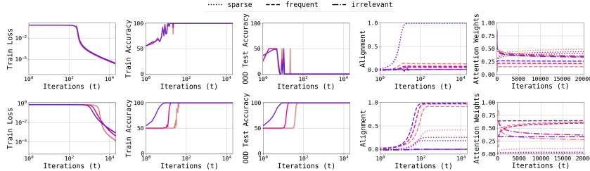
Figure 9: Train and test dynamics for a single-layer self-attention model (Eq. (3)) using the synthetic data visualized in Fig. 2; see Section 4.1 for details. The top row corresponds to the cases where the predictor that uses sparse tokens has lower sensitivity, while the bottom row corresponds to the cases where using the frequent tokens leads to lower sensitivity. The precise data settings for this figure, as well as a comparison of sensitivity values, are shown in Table 3.
