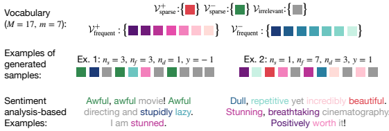
Figure 2: Visualization of the synthetic data generation process (see Section 4.1 for details). For simplicity, we represent each d -dimensional token with a square. Middle row: In each case, given a label y , we randomly sample T = 11 tokens, with n_s tokens from \mathcal{V}_{\text{sparse}}^y , \lfloor (n_f + n_d)/2 \rfloor tokens from \mathcal{V}_{\text{frequent}}^y , n_f - \lfloor (n_f + n_d)/2 \rfloor tokens from \mathcal{V}_{\text{frequent}}^{-y} and the remaining tokens from \mathcal{V}_{\text{irrelevant}} . Note that in the first example, since n_s = 3 and n_d = 1 , a predictor that relies (only) on the sparse tokens is less sensitive compared to the one that relies on the frequent tokens. On the other hand, in the second example, since n_s = 1 and n_d = 3 , the predictor that relies on the frequent tokens is less sensitive. Bottom row: We include two sentiment analysis-based examples to illustrate the synthetic data samples in the second row, using the same colors as the first two rows.
