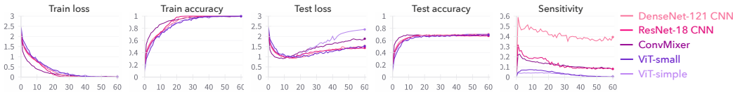
Figure 13: Comparison of the sensitivity of two CNNs, two ViTs, and ConvMixer trained on the CIFAR-10 dataset, as a function of training epochs. For a fair comparison, the figure also shows the train and test accuracies and loss values (cross-entropy loss). All models have similar accuracies but the ViTs have significantly lower sensitivity than the other models.
