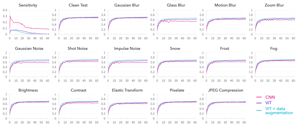
Figure 18: Comparison of the sensitivity, test accuracy on CIFAR-10, and test accuracies on various corruptions from the CIFAR-10-C dataset (see Section 7 for details) of a ResNet-18 CNN and a ViT-small model trained on the CIFAR-10 dataset, as a function of the training epochs. We also compare with ViT-small trained with data augmentation, which acts as a regularizer to encourage low sensitivity (see Section 7 for discussion). Here, we use severity level 1, while in Figure 17, we considered severity level 2.
