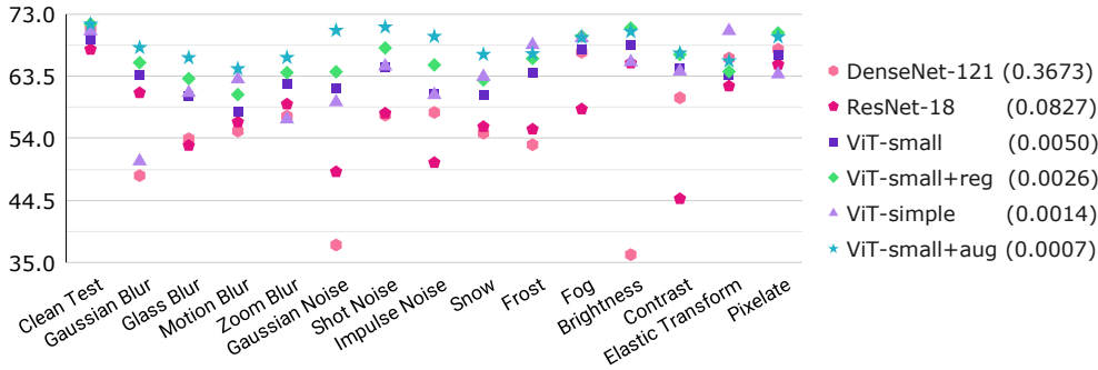
Figure 7: Comparison of the test accuracies on CIFAR-10 and on various corruptions from the CIFAR-10-C dataset (see Section 7 for details) of various models trained on the CIFAR-10 dataset, at the last training epoch (see App. Fig. 17 for a comparison of the accuracies as a function of training epochs.). We observe that the Vision Transformer models ViT-small and ViT-simple exhibit lower sensitivity and higher robustness to corruptions compared to the CNN models DenseNet-121 and ResNet-18. Additionally, encouraging lower sensitivity while training through regularization (ViT-small-reg) and data augmentation (ViT-small-aug) leads to improved robustness (see Section 7 for details).
