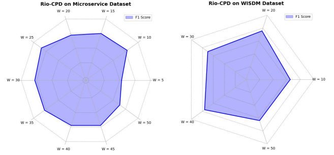
Figure 5: Sensitivity analysis of window size W for Rio-CPD.
