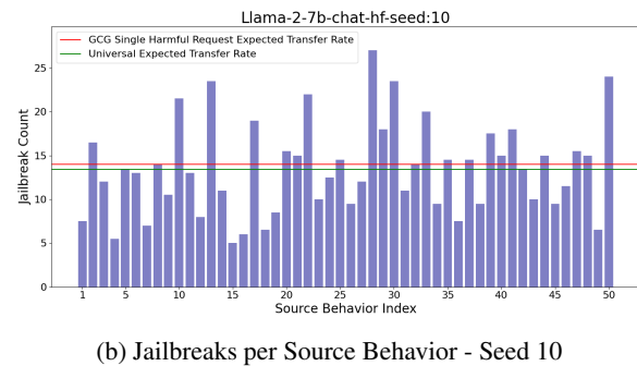
Figure 10: GCG Universal Attacks Across Source Behaviors and Models. Figures Fig. 10a and Fig. 10b represent GCG universal attacks where each bar indicates the number of jailbreaks each source behavior optimized by GCG achieves across five popular instruction-tuned open-source models. The high variance between the two figures illustrates that different source behaviors are responsible for the best universal suffix in each case.
