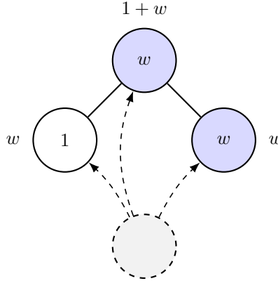
Figure IV.9: Illustration of the process at t = 3 with two vertices labelled w and one vertex labelled 1 . The attractiveness-weighted degree A_t of each of the existing vertices is displayed next to it. Up to normalization, these are the attachment probabilities for the new fourth vertex. TikZ figure produced by GPT-5.
