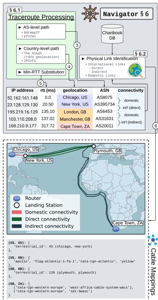
Figure 6: Overview of Calypso’s Navigator module
