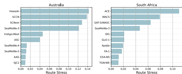
Figure 15: Route Stress values for case studies in Australia and South Africa.
