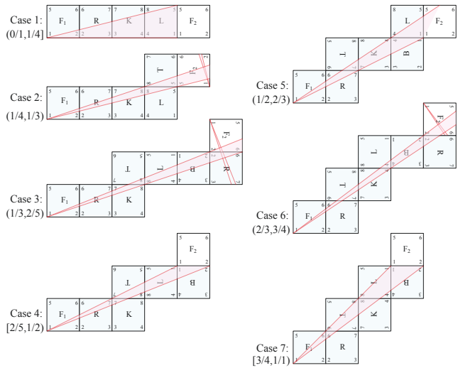
Figure 7: The seven slope cases, showing the range of slopes (in pink) progressing across the faces of the cube. The geodesic segment starts in face F_1 and revisits the starting face, marked F_2 (in white).
