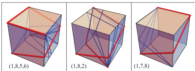
Figure 10: Red: Partial quasigeo, through vertices listed. Blue: All possible extension geodesic segments that pass the lengths ordering and the angle-turn eliminations, leaving only self-crossing to check.
