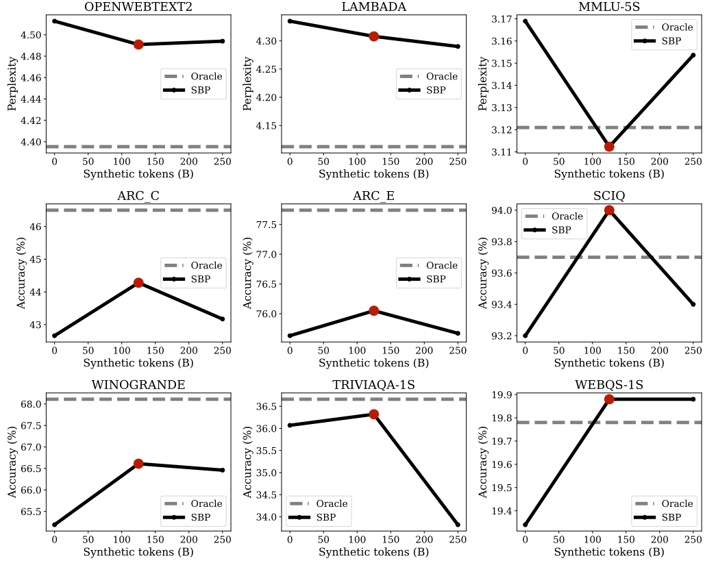
Figure 7: SBP performance with varying synthetic tokens at 1T-scale (3B).
